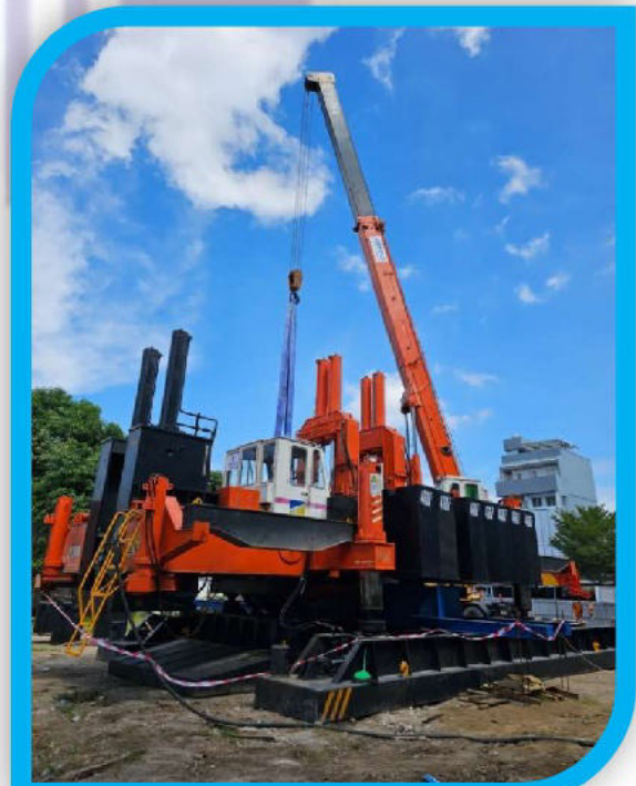
Hydraulic Static Pile Driver (HSPD) 460 Ton T-Work ZYC460B-CB1
